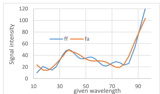
Figure. 1. Dependence of background f_f(\lambda_i) and reflected spectra on wavelength.
