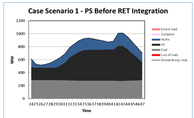
Figure 4: Daily generation profile before RET integration
