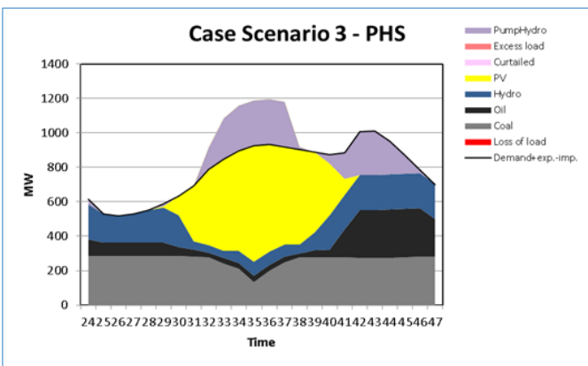
Figure 7: Daily generation profile after simulating PHS as solution to the duck curve
